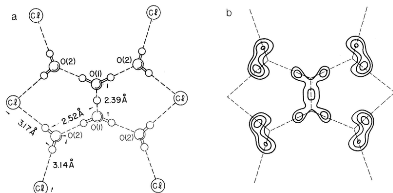
Fig. 2. (a) The H_{13}O_6^+ ion and the surrounding Cl^- ions. (b) Portions of a difference map, showing the electron density associated with the hydrogen atoms. Contours are drawn at 0.2, 0.3, and 0.4 electron/ \text{\AA}^3 .
